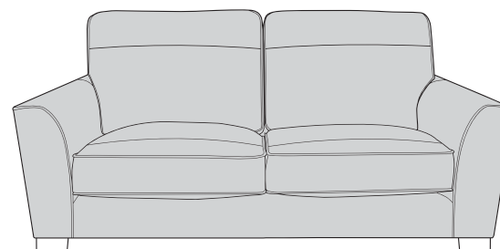
2 Seater Sofa: 2S H: 99 W: 182 D: 94
